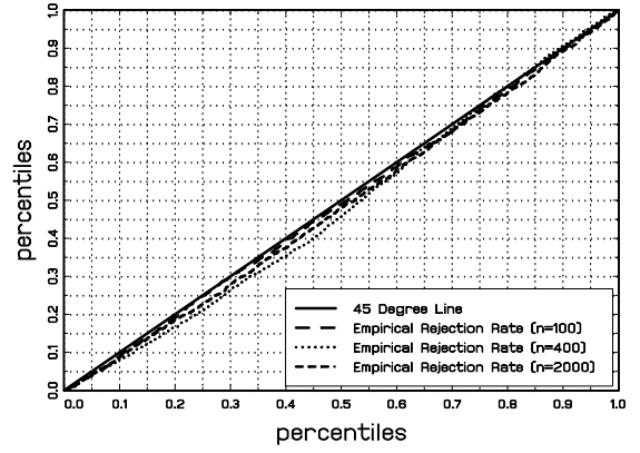
Figure 3: ESTIMATED p -VALUES OF THE QLR STATISTICS BY WEIGHTED BOOTSTRAP. Number of Replications: 2,000, DGP: Y_t = 0.5Y_{t-1} + U_t and U_t \sim \text{IID } N(0,1) , Model: Y_t = \alpha + \beta Y_{t-1} + \lambda \sin(\delta Y_{t-1}) + U_t , and K = 150
