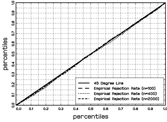
Figure 3: ESTIMATED p -VALUES OF THE QLR STATISTICS BY WEIGHTED BOOTSTRAP. Number of Replications: 2,000, DGP: Y_t = 0.5Y_{t-1} + U_t and U_t \sim \text{IID } N(0,1) , Model: Y_t = \alpha + \beta Y_{t-1} + \lambda \sin(\delta Y_{t-1}) + U_t , and K = 150
