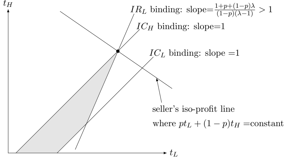
Figure 3: Set of feasible (t_L, t_H) for reverse screening menu with q_L and q_H given
