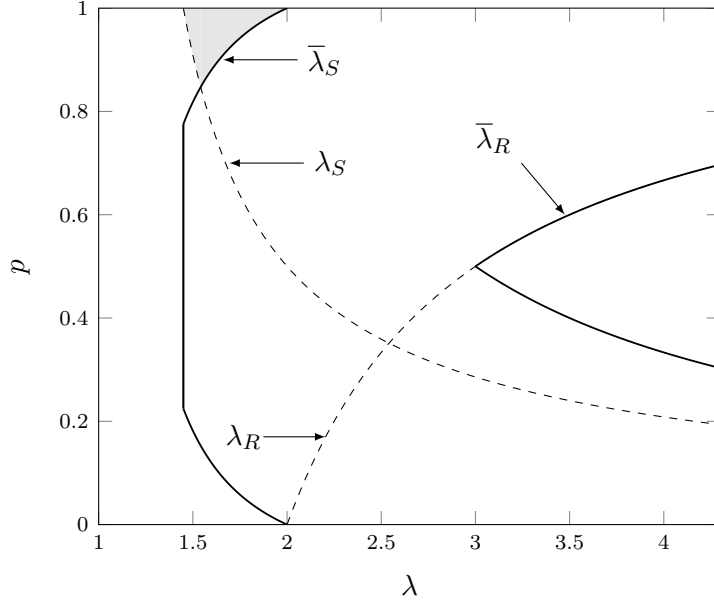
Figure 2: Optimal TPPE menu
