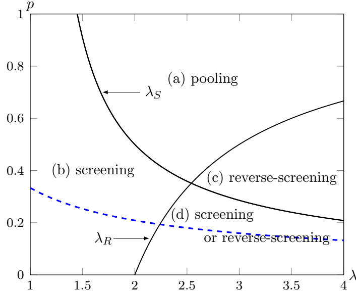
Figure 1: Optimal TPE menu
